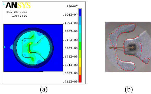
Fig. 6 Comparison of (a) simulated distribution of thermo-mechanical stress with (b) micrograph of delaminated lead frame.
