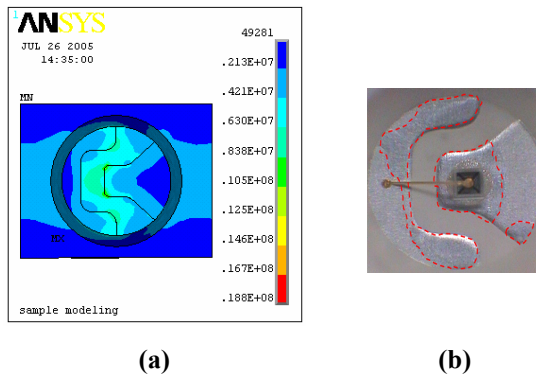
Fig. 10 Comparison of (a) simulated hygro-mechanical stress distribution with (b) micrograph of delaminated lead frame.
