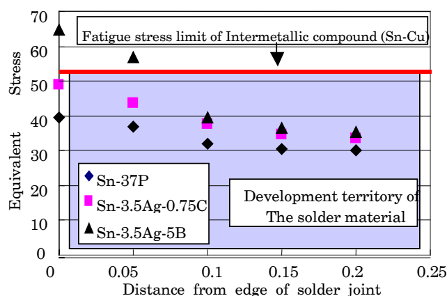
Fig.9 Distributions of Mises equivalent stresses
