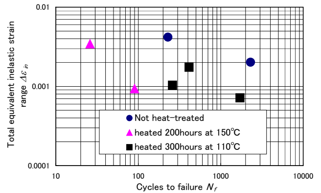
Fig. 6 S-N curves of Sn-8Zn-3Bi solder joints
