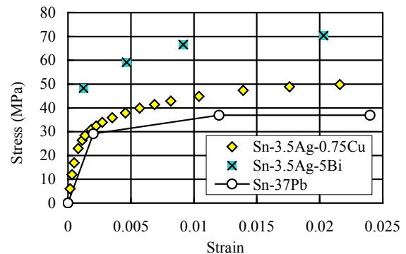
Fig.8 Stress-Strain curve of solder materials
