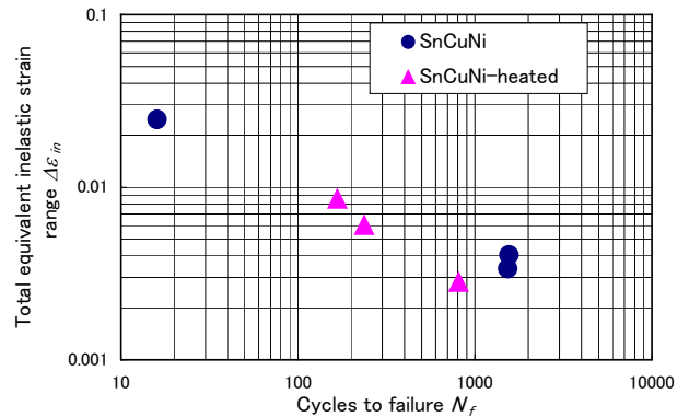
Fig.4 S-N curves of Sn-Cu-Ni solder joints
