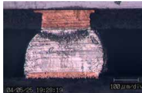
(b) Image of solder joint without void after test
