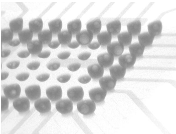
Fig.10 X-ray images of solder joint
