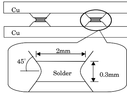
Fig.3 Structure of shearing type specimen
