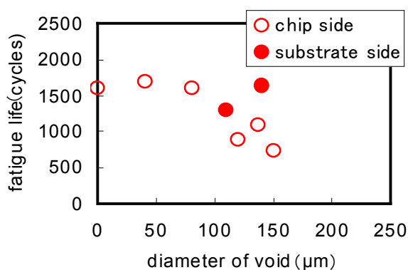
Fig.12 the relationship between fatigue life of solder joints and the position and size of the void in solder joints
