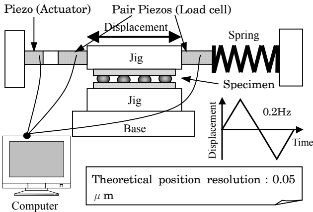
Fig. 2 Isothermal fatigue-testing equipment
