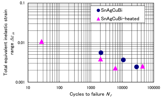
Fig. 5 S-N curves of Sn-2.9Ag-0.5Cu-3Bi solder joints
