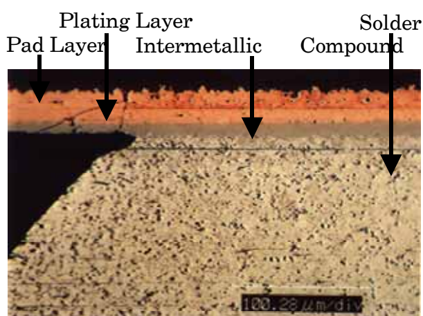
Fig.1 Structure of solder joint
