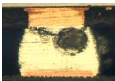
(a) solder joint with void formed on crack propagation route (void's \phi 140 \mu m fatigue life: 1100cycles)
