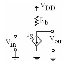
Figure 4: Simplified model of the considered amplifier.
