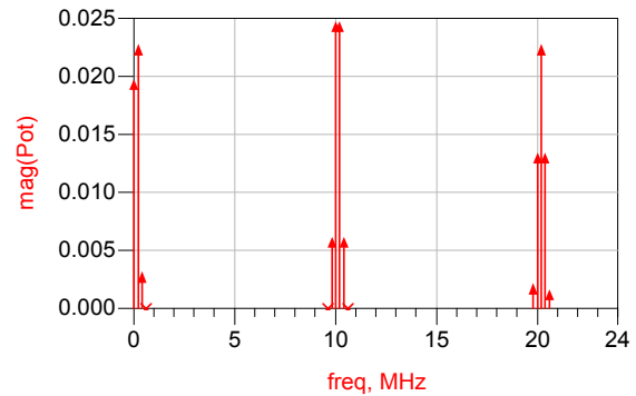
Figure 3: Spectrum of the dissipated power with some non-linear behaviour [W].
