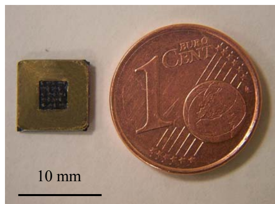
Figure 4: Membrane-electrode assembly (8×8 mm), scale comparison with a 1 cent euro coin.
