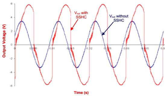
Figure 10 : The experimental results for SSHC technique.
