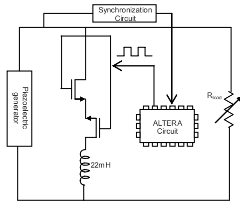
Figure 8 : The experimental realization of SSHI.
