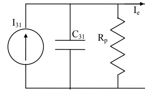
Figure 4 : The equivalent circuit of piezoelectric generator.
