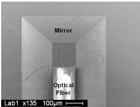
Figure 5. SEM micrograph of optical fiber inserted in silicon V-groove.
