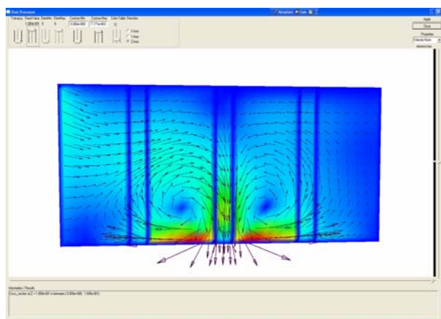
Figure.2. Velocity vector at the center of the microchannel with three driving electrodes
