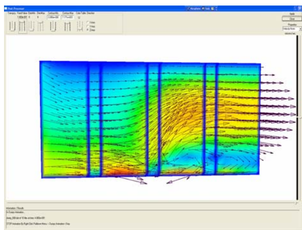
Figure. 3. The direction of the velocity vectors during a transient simulation of the EHD pumping principle.
