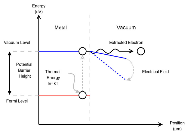
Figure 1 : Thermionic Emission Principle
