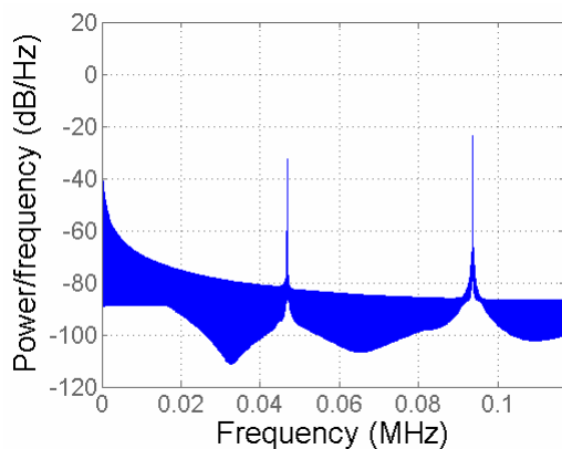
Figure 10. Bit stream spectrum corresponding to the same experimental conditions as in Figure 9.
