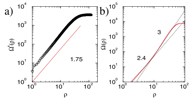
FIG. 4 (color online). Entanglement-entanglement correlation functions, \Omega , of the arrested state. (a) Single strand: 1/\nu_a^e = 1.75 ; (b) collective Hausdorff dimension of D_a^e = 2.4 .
