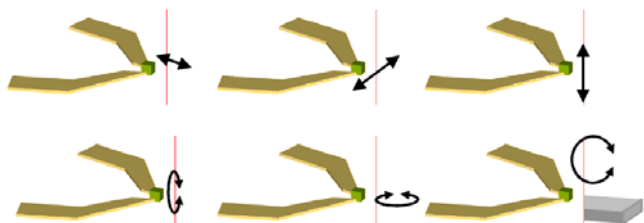
Fig. 6. Different degrees of freedom in 6 DOF microgripper [31].
