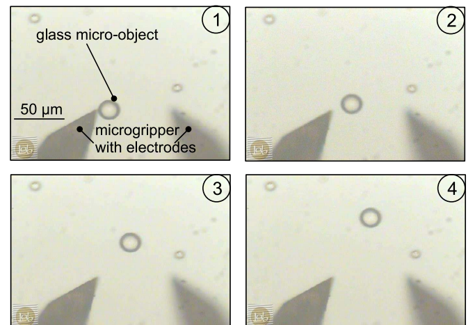
Fig. 9. Experimental DEP release
