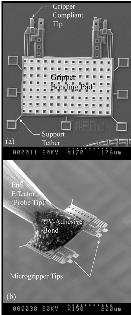
Fig. 4 SEM Image of Microgripper. (a) Microgripper on the Chip Substrate held by Tethers. (b) Microgripper Bonded with UV-Adhesive to the End Effector (Probe Pin) of the Micromanipulator.
