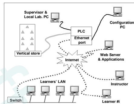
Fig 3: TIPY Architecture
