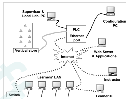
Fig 3: TIPY Architecture
