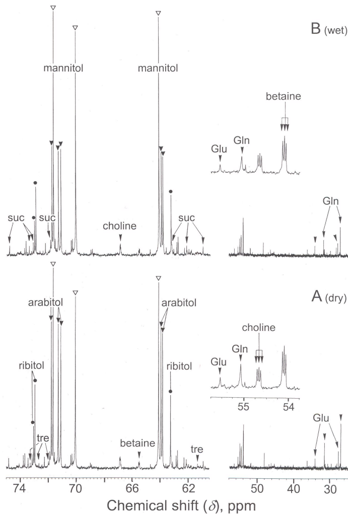
Fig. 5 Proton-decoupled ^{13}\text{C} -NMR spectra (100.6 MHz) of perchloric acid extracts of X. elegans thalli. PCA extracts were prepared from 4 g of thalli (on a dry weight basis) and analysed by ^{13}\text{C} -NMR. Thalli were collected as follows: A dry, in the light; B wet, in the dark. Peak assignments (from downfield to upfield): suc, sucrose; tre, trehalose; Glu, glutamate; Gln, glutamine. Spectra are representative of five independent experiments.
