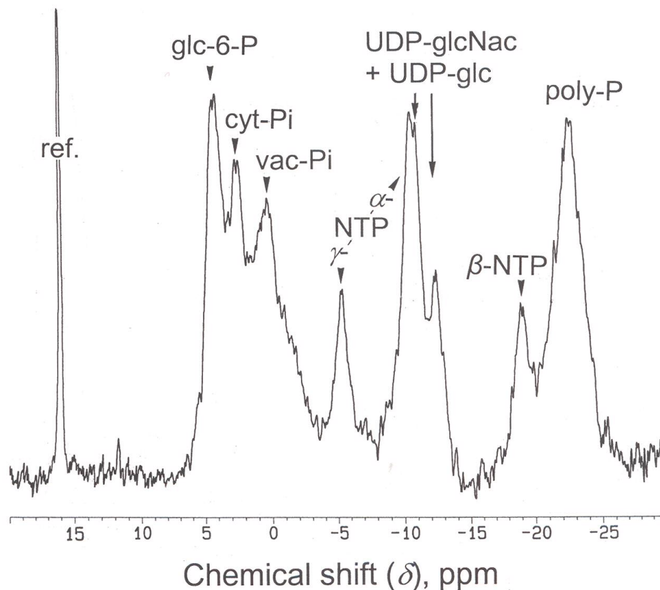
Fig. 4 Proton-decoupled in vivo ^{31}\text{P} -NMR spectrum of X. elegans thalli. Lichen fragments (4 g dry wt) were hydrated, packed in a 25 mm NMR tube as described in Gout et al. (2001), continuously perfused at a flow rate of 50 \text{ mL min}^{-1} with a well oxygenated medium containing 0.2 mM Mops buffer (pH 6.2), at 20^\circ\text{C} , and analyzed by ^{31}\text{P} -NMR. Peak assignments as in Fig. 2; cyt-Pi, cytoplasmic phosphate; vac-Pi, vacuolar phosphate; ref, reference.
