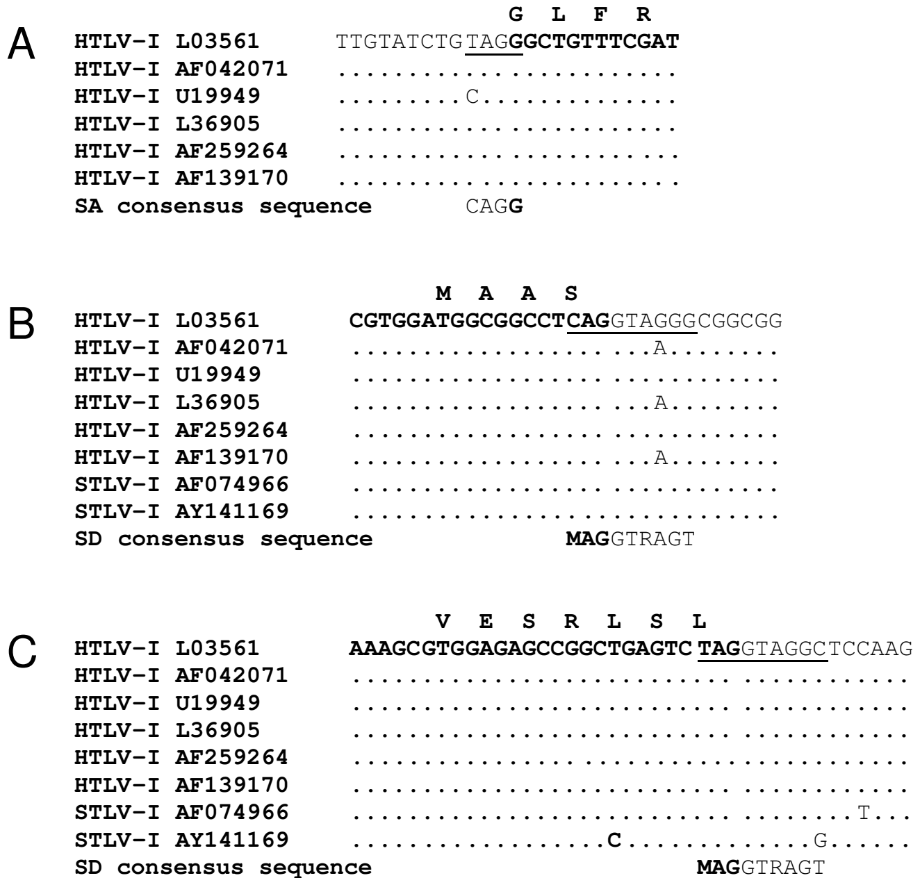
Figure 5 Sequence comparison of the HBZ splice acceptor, splice donors SD1 and SD2 and encoding regions between various HTLV-I and STLV-I isolates. STLV-I and HTLV-I sequences taken from GenBank were compared with different segments of the anti-sense strand of the K30 proviral DNA (accession number L03561 ): position 1756–1779 (splice acceptor) ( A ), position 350–379 (splice donor 1) ( B ) and position 182–239 (splice donor 2) ( C ). Comparisons were also made with the splice acceptor and splice donor consensus sequences (shown below compared stretches) and the corresponding K30 sequence is underlined. Coding regions are presented in bold and amino acid sequences are also indicated above the compared nucleotide sequence. GenBank accession numbers are provided for each compared STLV-I and HTLV-I proviral DNA clones.
