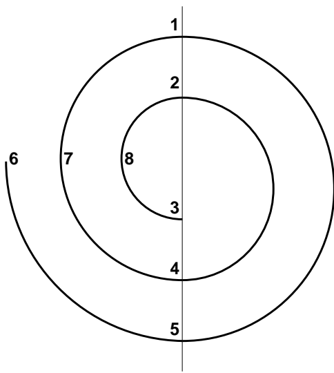
FIGURE 3. La 3-octine
