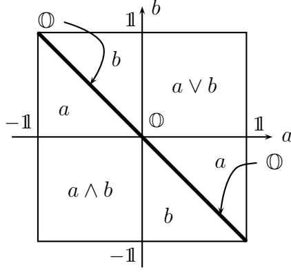
Fig. 1. Definition of the symmetric maximum a \oplus b
