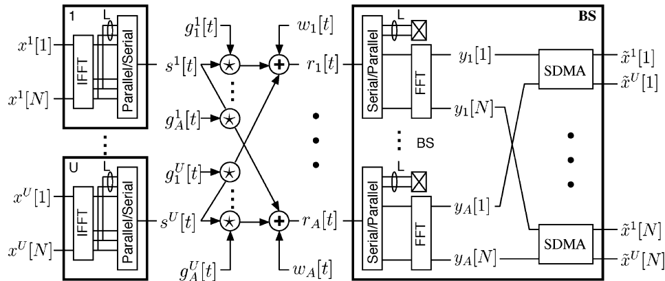
Fig. 1. System model for OFDM/SDMA in the uplink.
