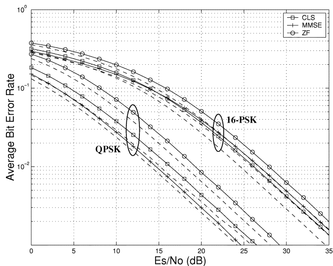
Fig. 9. Average BER versus SNR for OFDM/SDMA with channel estimation for K = 4 and U = 4 .
