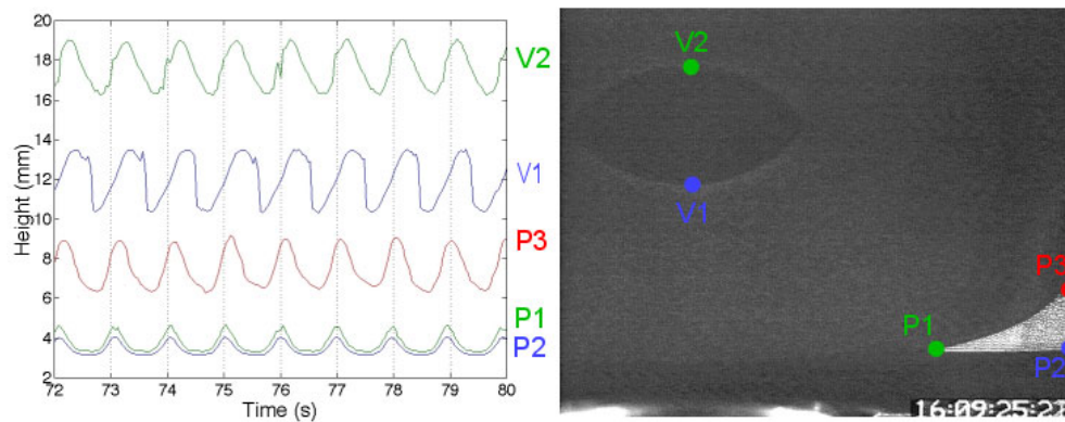
Figure 7. Time evolution of the height of characteristic points of the dust cloud under low frequency excitation (see also movie ).
