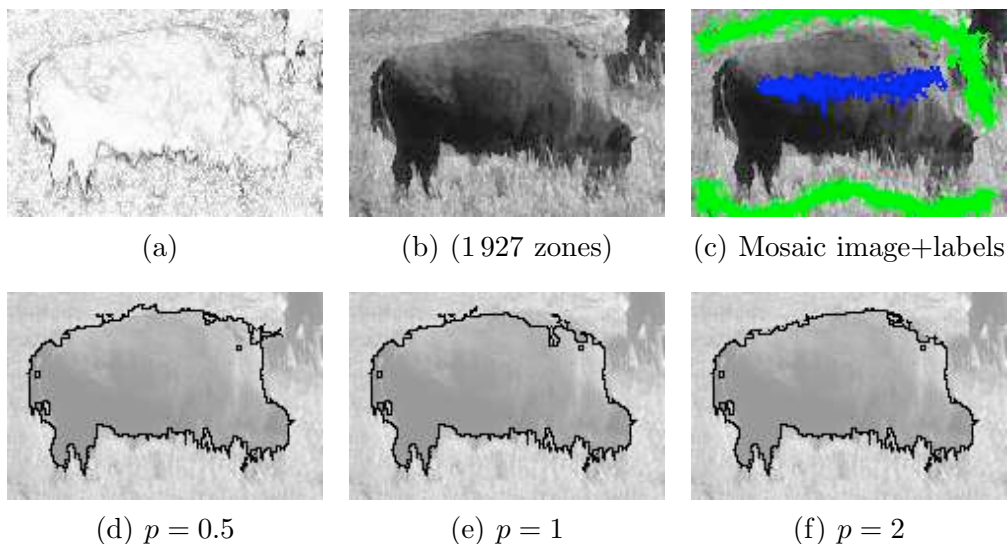
Fig. 5. Semi-supervised image segmentation based on the region adjacency graph of the mosaic image. The images are whitened for accentuate the labels and the segmented boundary. 5(a) energy image 5(b) mosaic image (1927 zones) from Fig. 4(a) (which contains 16 690 pixels) where each zone corresponds to the mean color model of the original image. 5(c) mosaic image with the user label 5(d), 5(e), and 5(f) segmentation results obtain with the corresponding p parameter.
