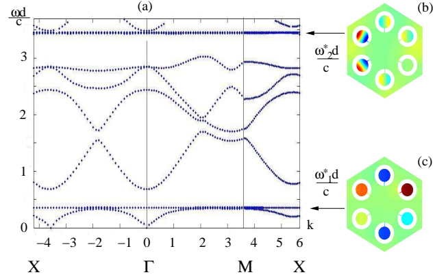
Fig. 2. Transverse incidence. (a) Dispersion diagram for six infinitely conducting inclusions shaped as split ring resonators of inner radius 0.159d and outer radius 0.259d (right) and filled with a dielectric material of relative permittivity 12. The center-to-center spacing of inclusions is 0.7d . Inclusions are surrounded by a matrix of relative permittivity 1. The horizontal axis shows the magnitude of the Bloch vector describing the first Brillouin zone described in Figure 1(c). On the vertical axis, we represent the eigenfrequencies of propagating TE waves. (b) Eigenfield associated with eigenfrequency \omega_1^* d/c = 0.35308 (root of multiplicity six) which is constant in the center of each C-shaped inclusion. (c) Eigenfield associated with eigenfrequency \omega_2^* d/c = 3.4540 (multiple root). We note the dipole nature of modes confined in the center of each C-shaped inclusion.
