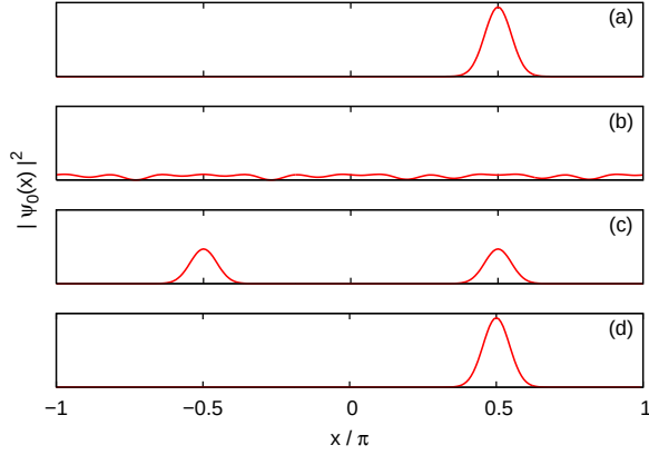
Figure 1: Free evolution of a localized wavepacket ( \beta = 0 ) between two successive kicks for \hbar = 4\pi . (a) Initial wavepacket centered at X = \pi/2 shown in the interval X \in [-\pi, \pi] , (b) wavepacket at t = 0.115 , showing complete delocalization, (c) wavepacket at t = 0.25 , showing two replicas of the initial shape, (d) “reconstructed” wavepacket at t = 1^- , identical to the initial one.
