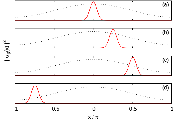
Figure 2: Wavepacket plotted at different integer times, for k = 4\pi and an irrational quasimomentum ( \beta = \frac{\pi}{50} \approx 0.063 ). (a) Initial wavepacket ( |\psi_\beta|^2 ) centered at X = 0 , (b) t = 1 , (c) t = 2 , (d) t = 5 . The shape of the potential is represented in dotted lines. The wavepacket interacts with the potential at different positions, and the average effect tends to zero.
