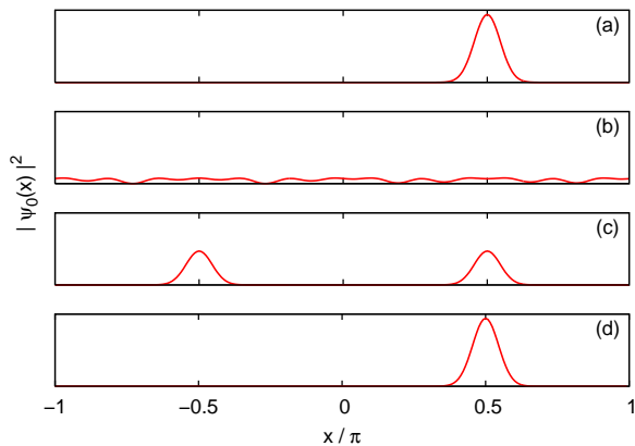
Figure 1: Free evolution of a localized wavepacket ( \beta = 0 ) between two successive kicks for \bar{k} = 4\pi . (a) Initial wavepacket centered at X = \pi/2 shown in the interval X \in [-\pi, \pi] , (b) wavepacket at t = 0.115 , showing complete delocalization, (c) wavepacket at t = 0.25 , showing two replicas of the initial shape, (d) “reconstructed” wavepacket at t = 1^- , identical to the initial one.
