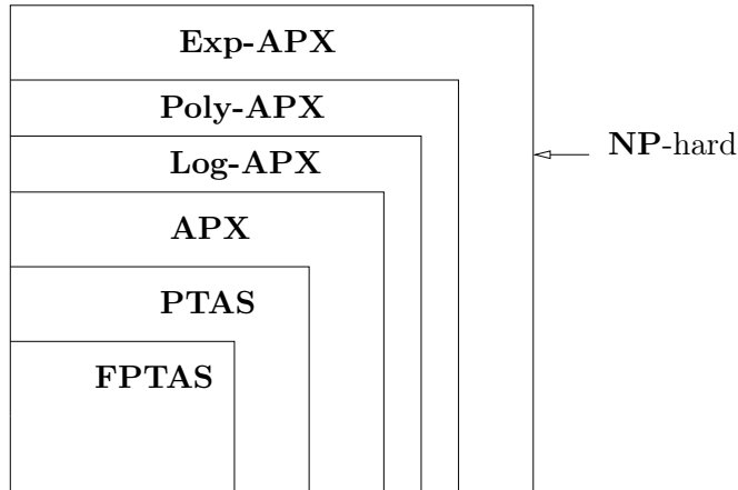
Figure 1: Standard approximability classes (under the assumption \mathbf{P} \neq \mathbf{NP} ).
