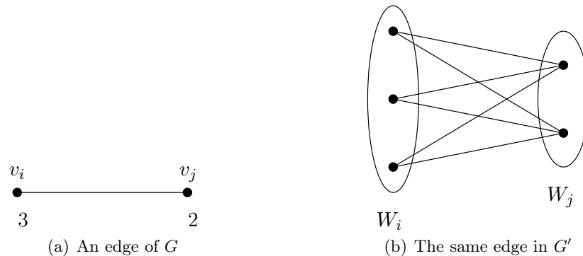
Figure 11: Transformation of an instance (G(V, E), \vec{w}) of MAX WEIGHTED INDEPENDENT SET into an instance G'(V', E') of MAX INDEPENDENT SET.
