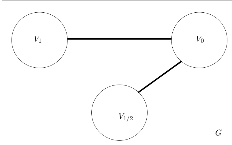
Figure 3: A graph G , input of MAX INDEPENDENT SET, and the possibility of existence of edges between sets V_0 , V_1 and V_{1/2} computed by the solution of MAX INDEPENDENT SET-R.
