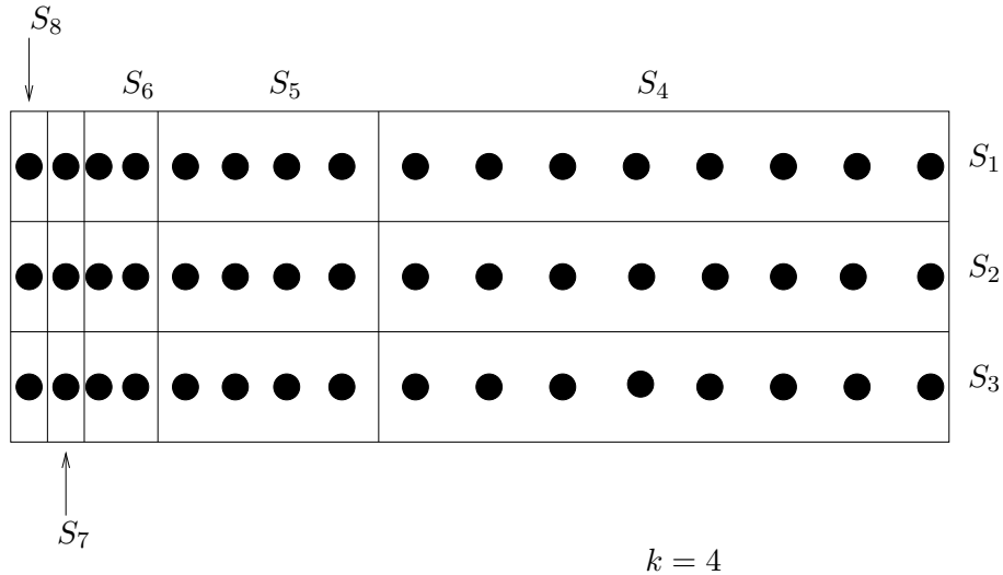
Figure 4: On the tightness of GREEDYSC with k = 4 .
