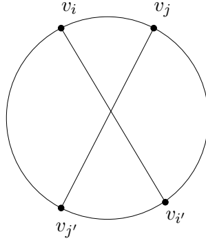
Figure 6: Algorithm 2_OPT
