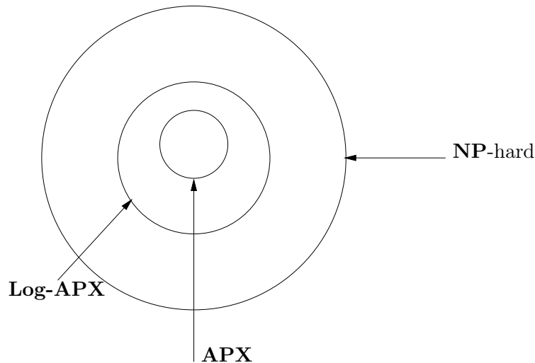
Figure 10: Designing an approximability hierarchy for NP -hard class.
