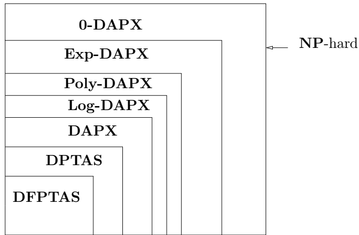
Figure 2: Differential classes (under the assumption \mathbf{P} \neq \mathbf{NP} ).
