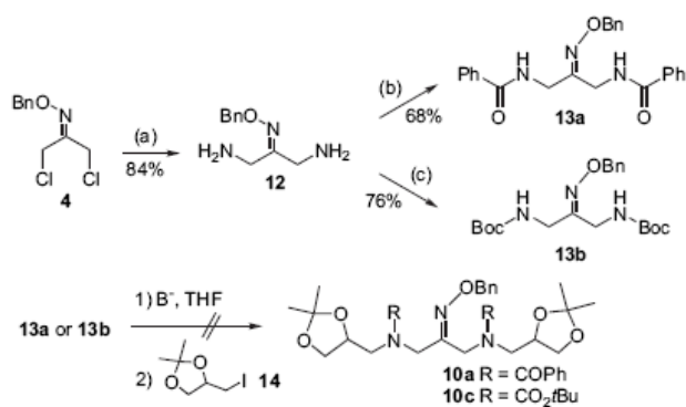
Scheme 4. Reagents and conditions: (a) PhNK, DMF, reflux then NH 2 –NH 2 , MeOH, reflux; (b) PhCOCl, NEt 3 , DMAP, CH 2 Cl 2 , 0 °C then 20 °C; (c) (Boc) 2 O, Na 2 CO 3 , dioxane, 20 °C.
