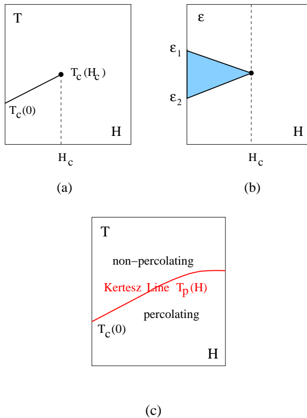
Figure 1: Thermodynamic and geometric phase structure for a first order transition
