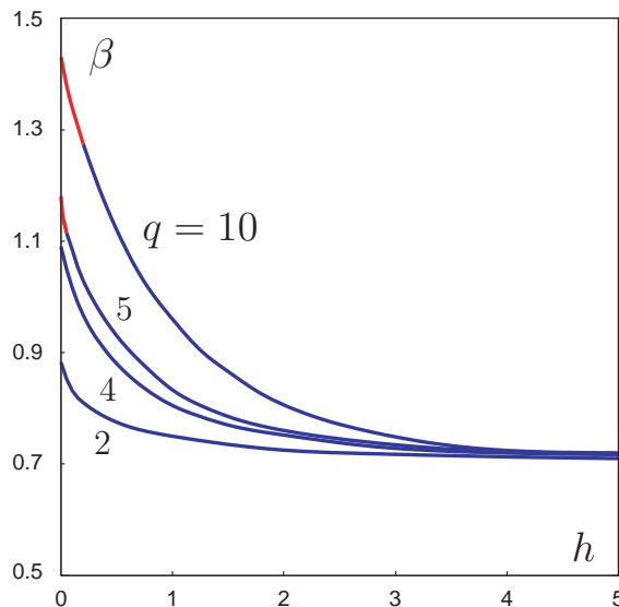
Figure 3: \beta_c(h) for several values of q , with “first order” behavior in red, “second order” in blue. The first order behavior is both thermodynamic and geometric. The second order behavior is only geometric.
