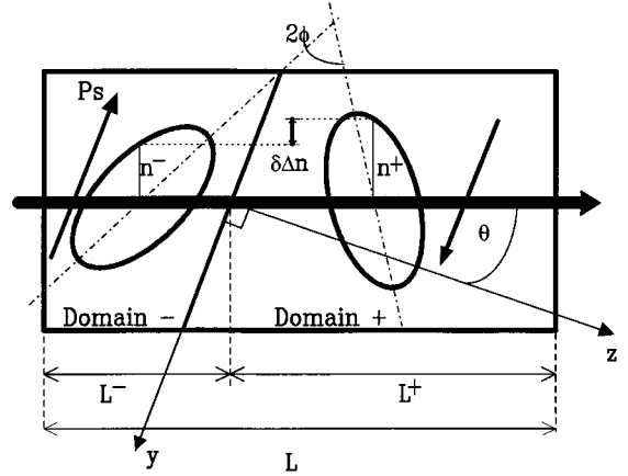
Fig. 5. Indicatrix cross sections in neighboring domains of RHSe in the (y, z) plane (the tilt angle \phi is voluntarily exaggerated). The tilt gives rise to a difference of birefringence between opposite domains, provided that the propagation direction is not perpendicular to the domain walls.
