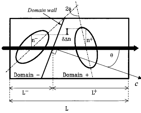
FIG. 6. Mutual tilt of the optical indicatrices in neighboring domains. When the propagation direction of the light is not perpendicular to domain walls, the birefringences \Delta n^+ and \Delta n^- in neighboring domains are different.
