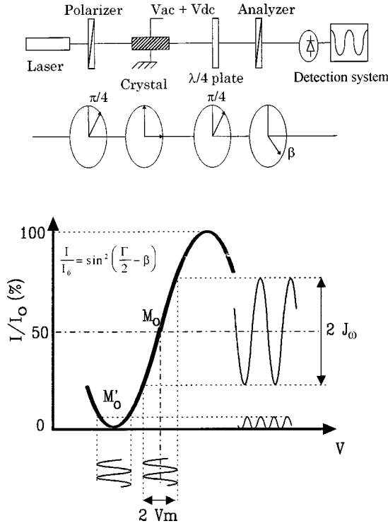
FIG. 1. S  narmont's setup used for electro-optic and birefringence cycle measurements (upper part). Transmission factor corresponding to this optical arrangement showing two particular working points M_0 and M'_0 (lower part).
