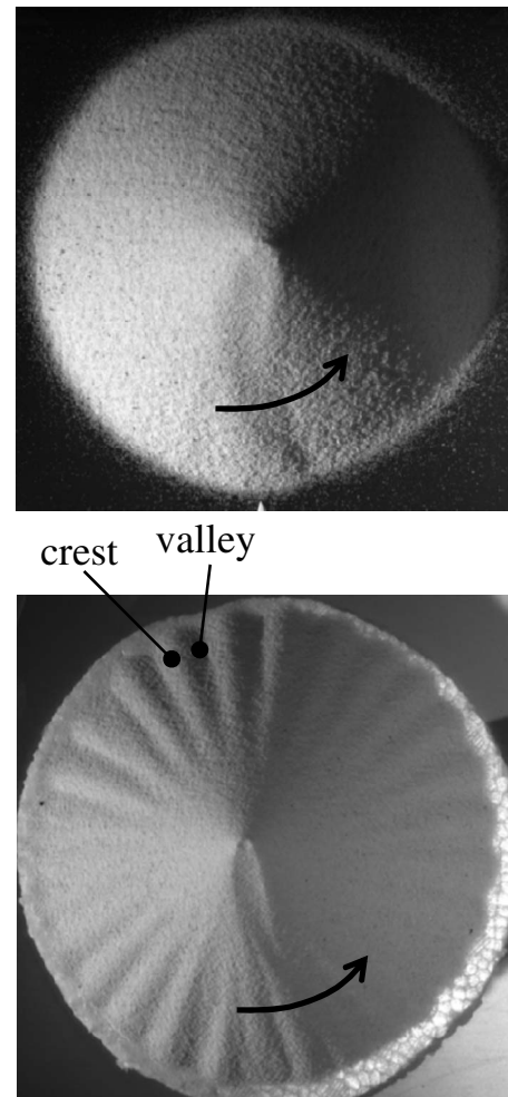
FIG. 2. Topography of the continuous and intermittent regimes. Upper panel: Top view showing a pile “frozen” during a continuous river experiment. The diameter of the pile is 11 cm. Lower panel: Top view of a pile “frozen” during an intermittent river experiment. The diameter of the pile is 17 cm—surface undulations extend approximately 6 cm from the edge of the pile in the radial direction. Black arrows on top of the flowing river indicate the direction of revolution of the rivers as sand is added from above.
