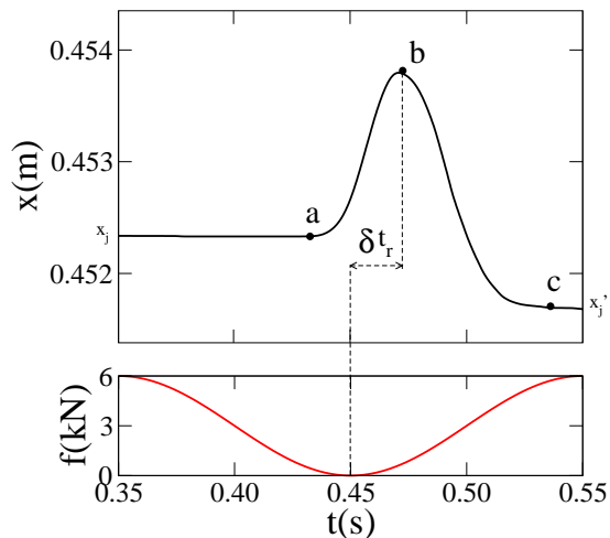
Fig. 5. A zoom on the displacement of the free wall as a function of time for a single period (up) in response to harmonic force (down).
