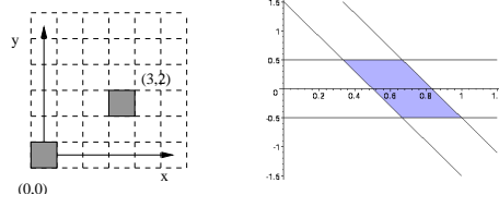
Fig. 1. An example of \mathcal{S}(s, t) domain with pixels (0,0) and (3,2) , the \mathcal{S}(s, t) domain in the parameter space defined by inequations : \{\beta < 1/2, \beta \geq -1/2, \beta < -3\alpha + 5/2, \beta \geq -3\alpha + 3/2\} .
