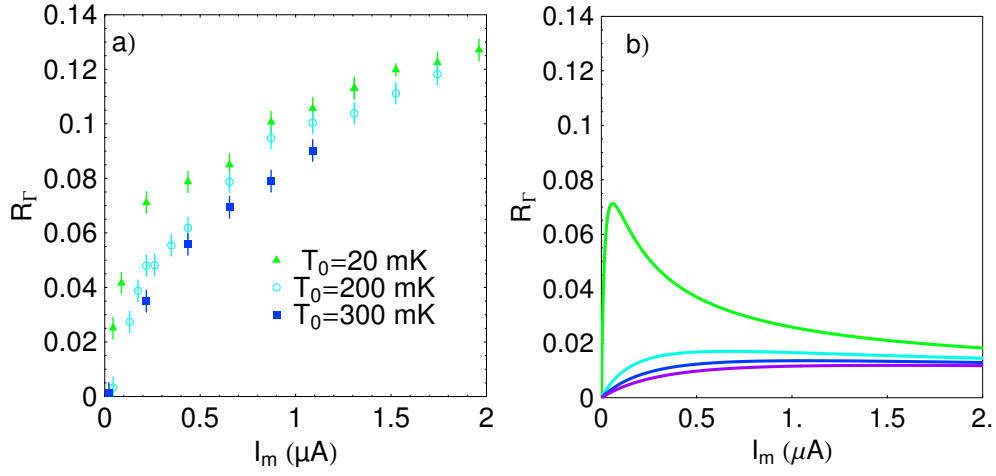
Fig. 8 a) Measured asymmetry R_T as function of the current I_m at a fixed value of the exponent B = 10.5 in the rate (1) for various temperature. b) Same quantity calculated using (11), assuming the actual temperature is the refrigerator temperature.
