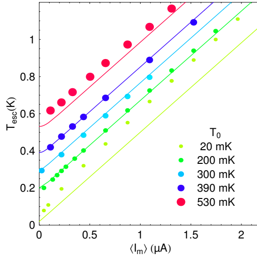
Fig. 5 Escape temperatures extracted using Eq. 1 (with I_0 = 479 nA, C = 36 pF) from the measurement of the rate as a function of s for several values of the current in the tunnel junction I_m and of the refrigerator temperature T_0 . The lines show the behavior expected from Eq.(3), in which a = eR_{||}/2k_B was taken as a fit parameter ( a_{fit} \simeq 0.48 K/ \mu\text{A} ).
