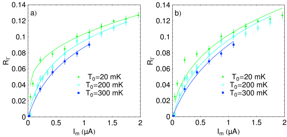
Fig. 9 a) Plot of the asymmetry R_T for a fixed value B = 10.5 assuming that the actual value of the current s is given by s \leftarrow s \pm \lambda \langle I_m \rangle / I_0 because of a possible leak through the capacitor C_1 . Besides, the temperature \theta_{\text{eff}} was extracted from Fig.5 instead of being calculated from Eq.(9). Here, \lambda = 5.5 \times 10^{-4} leads to the best fit with the data. b) Same thing assuming that the third moment is 0, that is g = 0 . Here, \lambda = 7 \times 10^{-4} leads to the best fit with the data.
