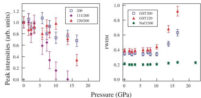
FIG. 2 (color online). Peak area (left) and peak FWHM (right) variation with pressure. The unchanged NaCl peak width indicates that hydrostatic conditions are preserved throughout the pressure range used.
