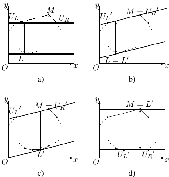
Figure 8. What may happen if M is above (U_LU_R) and after L .
