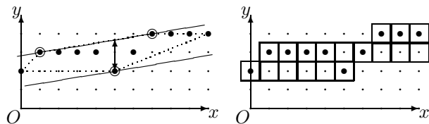
Figure 3. The optimal bounding line \mathcal{D}(1, 6, 0, 11) (squares) of a blurred segment S (black disks) of width \nu = 2 .
