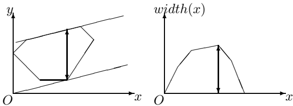
Figure 5. Vertical width and width function.
