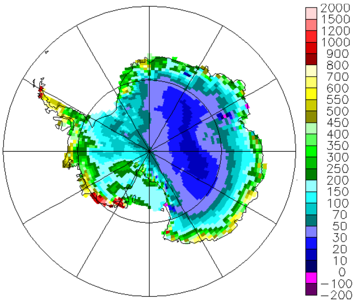
Figure 2. Simulated Antarctic Ice Sheet SMB ( \text{kg m}^{-2} \text{yr}^{-1} ) for the years 1981 to 2000.
