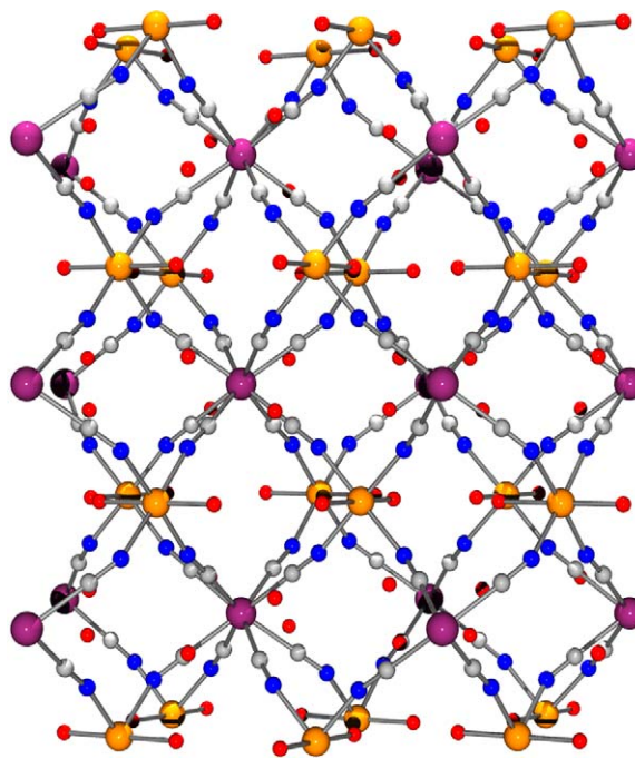
Fig. 1. View of the 3D arrangement of [\{\text{Co}(\text{H}_2\text{O})_2\}_2\text{Mo}(\text{CN})_8] \cdot 4 \text{H}_2\text{O} down the b direction.
