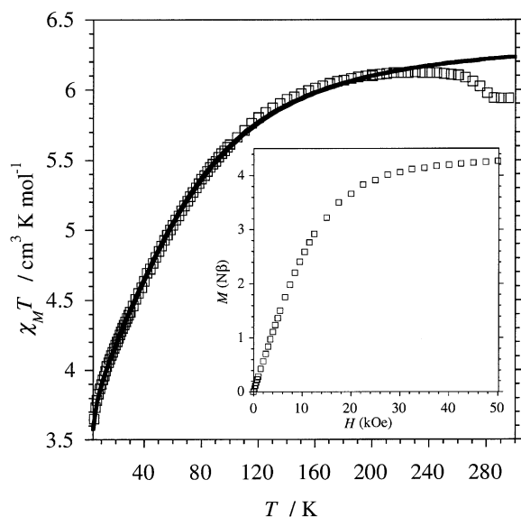
Fig. 4. Temperature dependence for the experimental ( \square ) and calculated (—) \chi_{\text{M}}T for [\text{Co}(\text{H}_2\text{O})_2]_2\text{Mo}(\text{CN})_8 \cdot 4\text{H}_2\text{O} yielding g = 2.604 \pm 0.001 , D = -80.3 \pm 0.6\text{ cm}^{-1} and \theta = -0.36 \pm 0.01\text{ K} . Insert: Field dependence of the magnetization recorded at 2 K.
