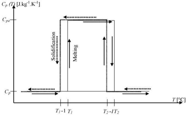
Fig. 10. Specific heat capacity as a function of temperature used in Type 101.
