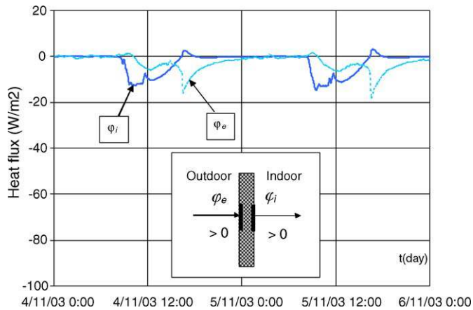
Fig. 7. Test-cell without PCM: heat flux variation, external ( \varphi_e ) and internal ( \varphi_i ). The positive direction of flux is shown in the inset.
