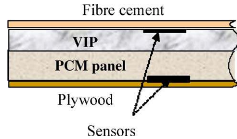
Fig. 5. Location of sensors of flux/temperature on the panels with PCM (same location for the panels without PCM).
