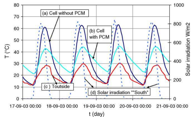
Fig. 6. Thermal behaviour of the two test-cells (without and with PCM): (a) indoor temperature variation of the cell without PCM, (b) indoor temperature variation of the cell with PCM, (c) outdoor temperature variation and (d) solar irradiation (vertical, south orientation).
