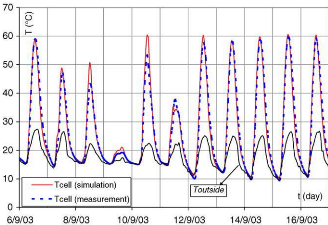
Fig. 11. Comparison of simulated and measured indoor temperatures of the test-cell without PCM during 10 days of September.
