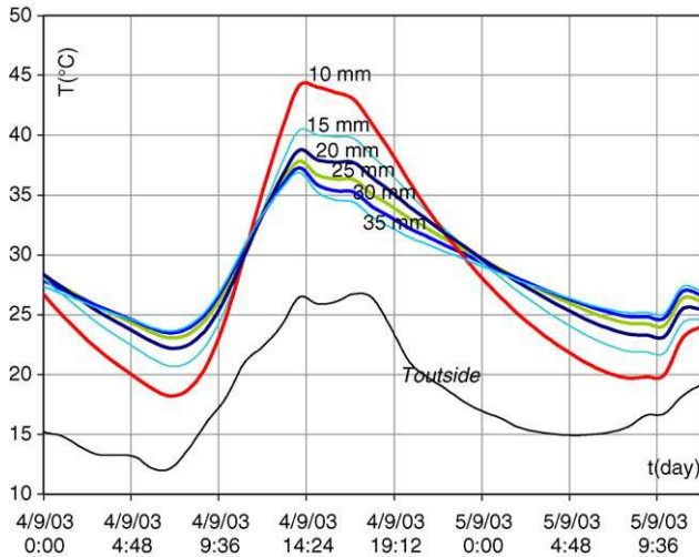
Fig. 14. Influence of wallboard thickness on the inside temperature of a test-cell with PCM for real climatic conditions.
