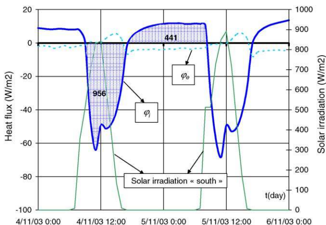
Fig. 8. Test-cell with PCM: heat flux variation, external ( \varphi_e ) and internal ( \varphi_i ).
