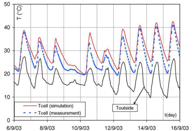
Fig. 13. Comparison of simulated and measured indoor temperatures of the test-cell with PCM during 10 days of September.
