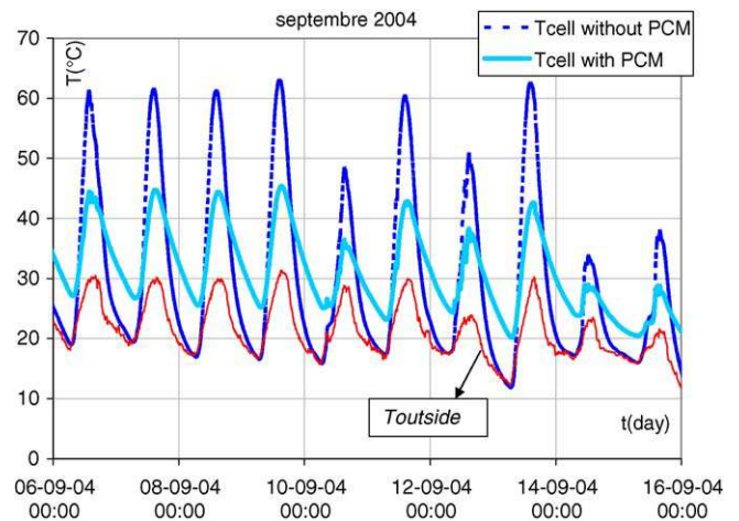
Fig. 9. Inside temperature of the two test-cells (without and with PCM) for September 2004.
