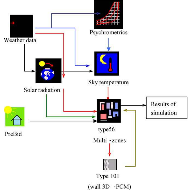
Fig. 12. Diagram for the PCM test-cell simulation showing the links between the different components under IISiBat interface.
