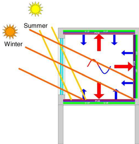
Fig. 3. Principle of solar heating of test-cells.
