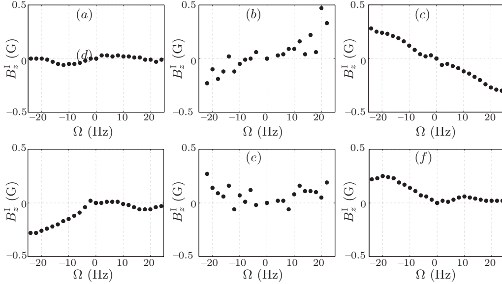
Fig. 6. Induced axial magnetic field when a 1000 A axial current passes through the vessel. Measurements are made at point 1 (upper row) and point 2 (lower row) for the flow driven by the rotation of disc 1 alone (left panels), disc 2 alone (right panels), or both counter-rotating discs (center).
