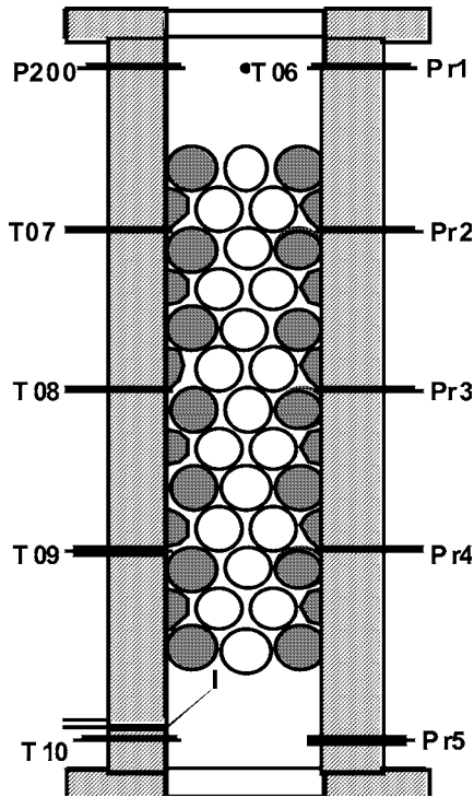
Fig. 2. Test section.
