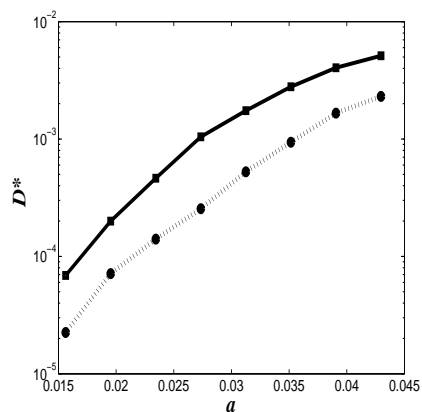
Fig. 4. Test particle diffusion coefficient D^* versus a (magnitude of the potential) in log-lin scale obtained for the turbulent potential V without (full squares, solid line) and with (full circles, dashed line) the addition of the control term f_2 given by Eq. (10).
