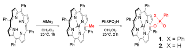
Figure 1. Synthesis of the complexes 1 and 2.
