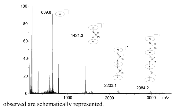
Figure 6. FAB + mass spectrum of the complex 2 . The different fragments
