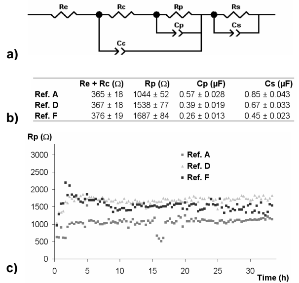
Fig. 6: EIS experiments a)Equivalent circuit b)Table result c) R_p measurement, see Table1 for Ref. details.
