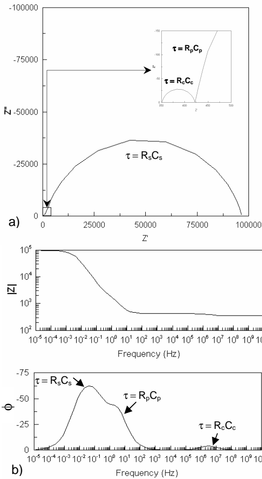
Fig. 5: Electrochemical response of alumina composite a)Nyquist and b)Bode diagrams
