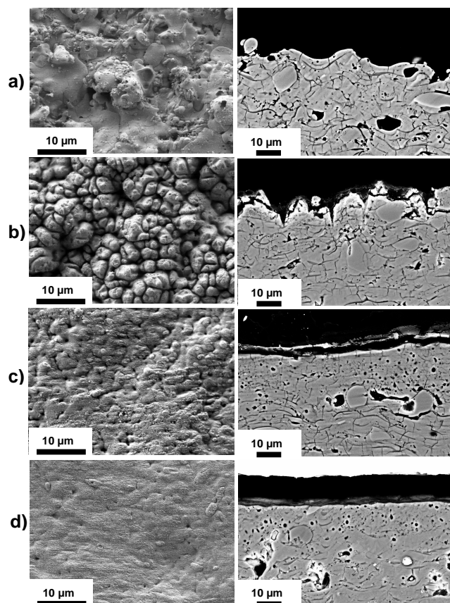
Fig. 3: Composite microstructures a) As-sprayed alumina surface and cross section b) 2\text{J}\cdot\text{cm}^{-2} - 500 pulses :Crater formation and crater cross-section c) 6.2\text{J}\cdot\text{cm}^{-2} - 250 pulses: surface and cross section d) 8\text{J}\cdot\text{cm}^{-2} - 250 pulses: surface and cross section.
