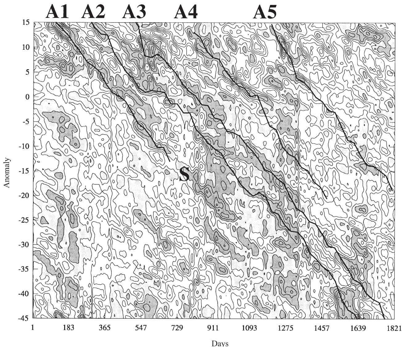
Figure 10. Time-longitude diagram of the upper-layer transport anomalies (in Sv), averaged between 27^{\circ} S and 35^{\circ} S. Time unit is in days. Contour interval is 1 Sv. Positive (anticyclonic) anomalies are in light grey, and anomalies larger than 1 Sv in dark grey. Positions (in longitude) of the five eddies are indicated with thick lines.
