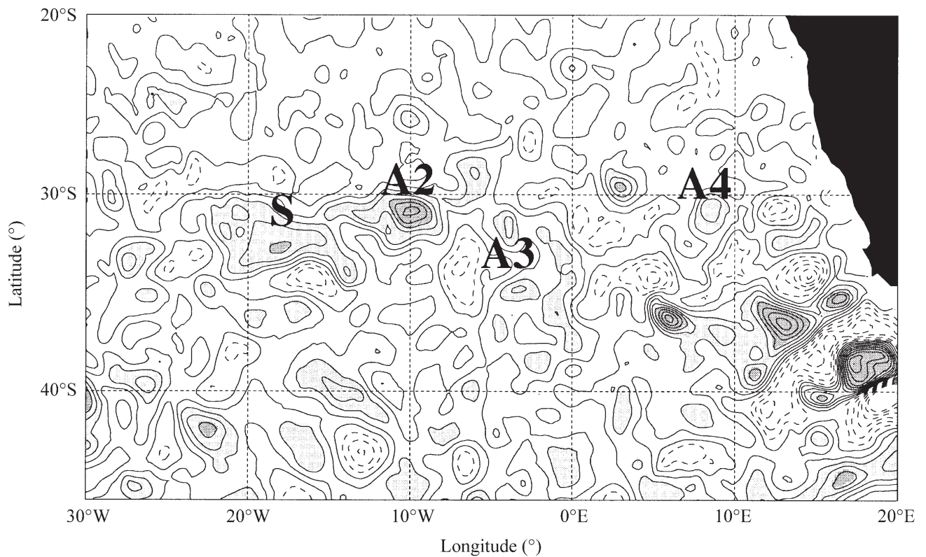
Figure 8. Map of sea-level anomalies in the Retroflexion region and the eastern Subtropical Gyre, as produced by the assimilation experiment on 19 March 1995. Contour interval is 5 cm, negative values are dashed. Anomalies larger than 10–20 cm are coloured in light/dark grey.
