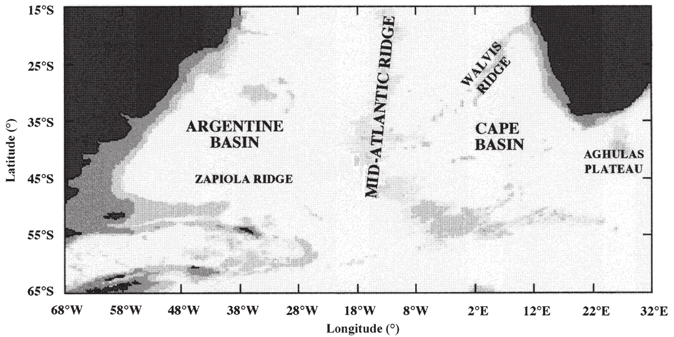
Figure 3. Sketch of the South Atlantic bathymetry with indications of the name locations of the main topographic features that are mentioned in the text.
