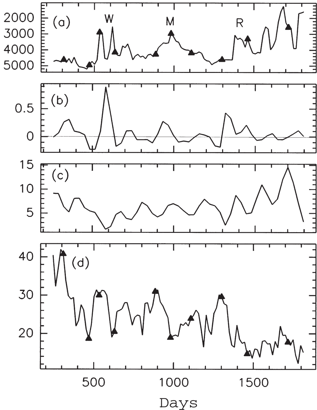
Figure 13. Time series of (a) the bathymetry (in m) over which eddy A2 passes, averaged over 1^\circ \times 1^\circ bins. Topographic ridges are indicated: Walvis Ridge (W), Mid-Atlantic Ridge (M) and Rio Grande Rise (R); (b) the decay rate of eddy height with distance (in \text{mm km}^{-1} ); (c) the phase speed (in \text{cm s}^{-1} ); (d) the maximum eddy height (in cm). Triangles indicate the positions of the eddy at the times corresponding to figure 11.
