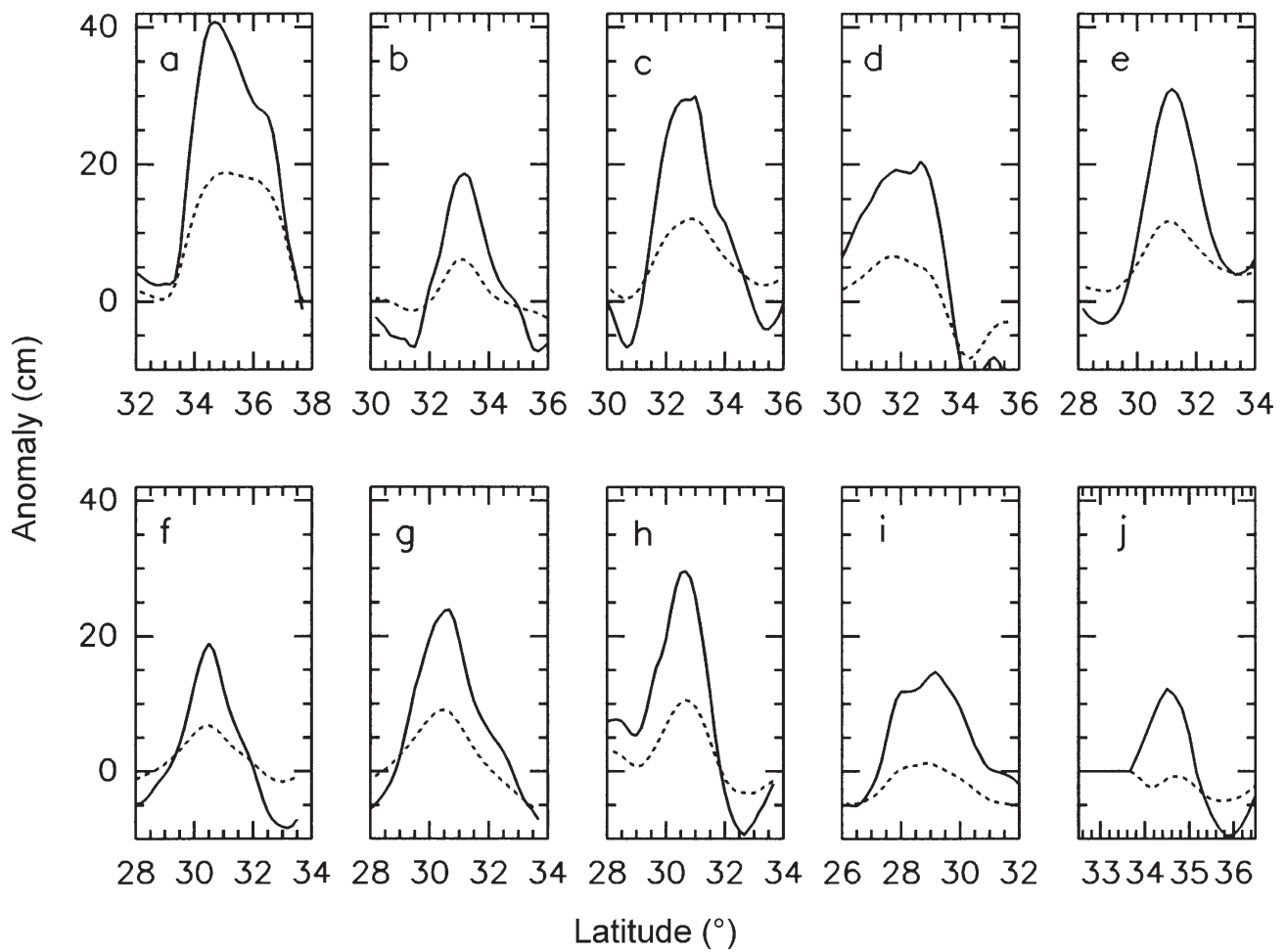
Figure 11. Sea-level anomaly (in cm) across eddy A2 (solid line), at the positions indicated on figure 12. (a) 6 August 1993; (b) 12 January 1994; (c) 16 March 1994; (d) 21 June 1994; (e) 4 March 1995; (f) 8 June 1995; (g) 14 October 1995; (h) 24 April 1996; (i) 2 October 1996; (j) 16 June 1997. Dotted line corresponds to the equivalent anomaly in layer 3 ( f_0/g \cdot \psi'_3 ).
