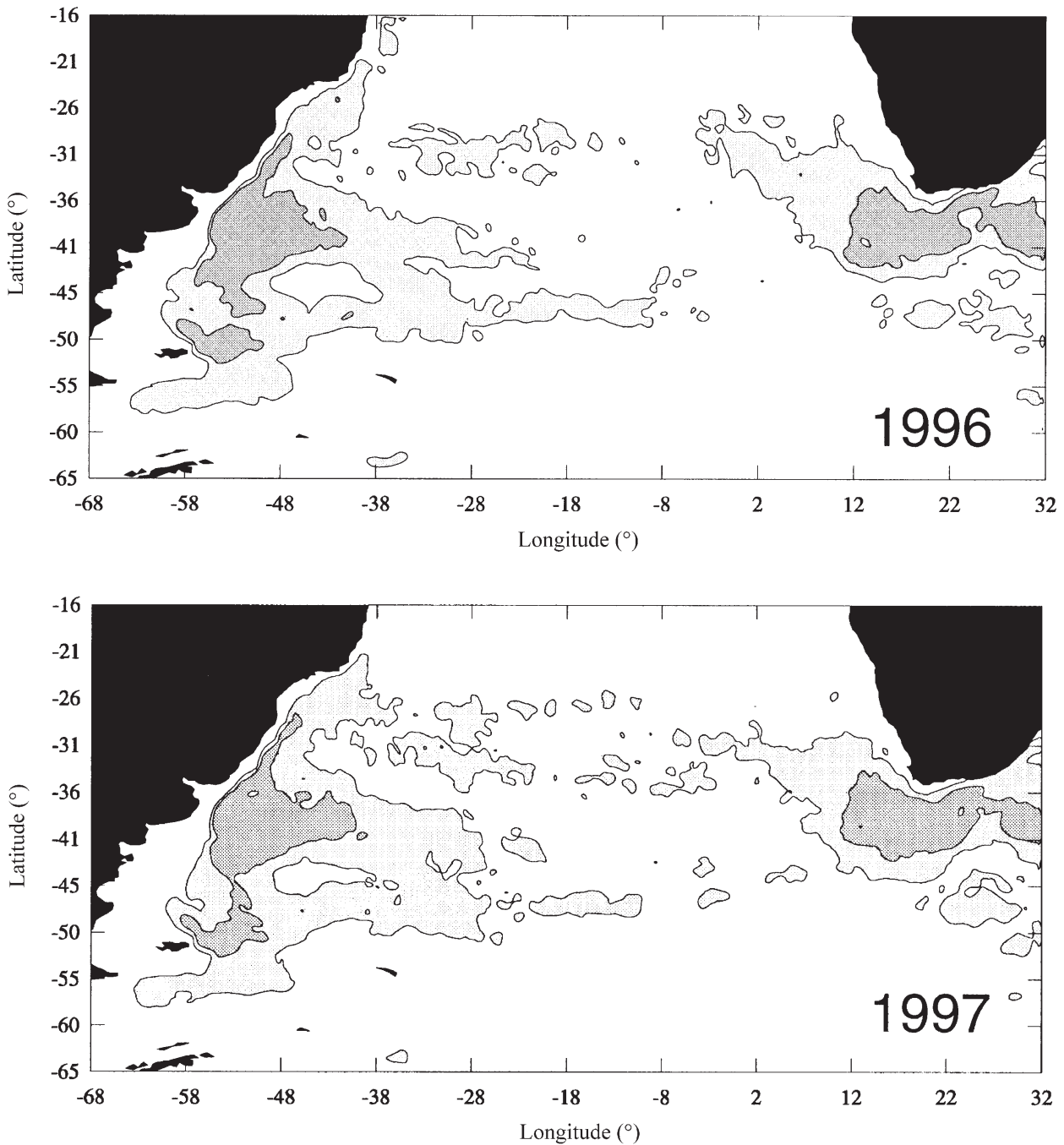
Figure 7. Annual mean eddy-kinetic energy for the 5 years of the experiment. Values larger than 80/300 \text{ cm}^2 \text{ s}^{-2} are coloured in light/dark grey.
