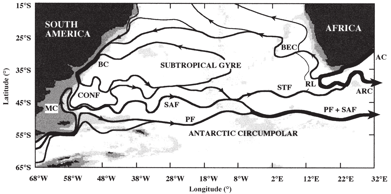
Figure 2. Sketch of the South Atlantic surface mean circulations: abbreviated terms are, BC, Brazil Current; MC, Malvinas Current; CONF, Confluence of the Brazil and Malvinas currents; AC, Agulhas Current; ARC, Agulhas Retroflexion; PF, Polar Front; SAF, Subantarctic Front; STF, Subtropical Front; BEC, Benguela Current and Retroflexion loop (RL).
