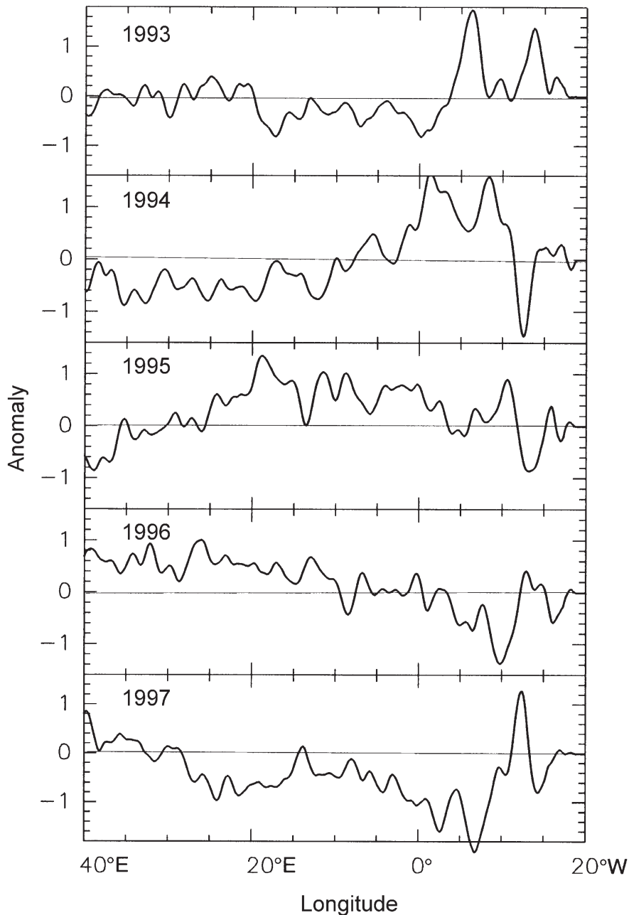
Figure 6. Annual mean anomalies of the upper-layer transport (in Sv) averaged over the ( 27^{\circ}\text{S} – 35^{\circ}\text{S} ) latitudinal band, as a function of the longitude.
