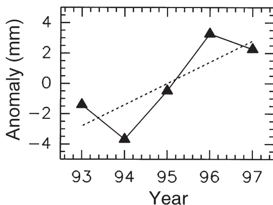
Figure 4. Annual mean sea-level anomalies, averaged over the domain for the 5-year experiment. The best-fit straight line (dotted) gives a global mean sea-level increase of 1.4 \text{ mm year}^{-1} .
