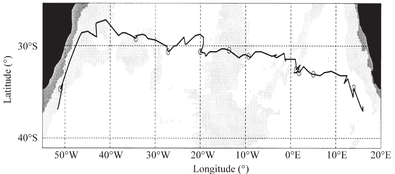
Figure 12. Drift path of eddy A2 as produced with an eddy-tracking time interval of 16 days. Circles indicate the positions of the eddy at the times corresponding to figure 11. Note the more complicated trajectory than with a 32-day interval (see figure 9).
