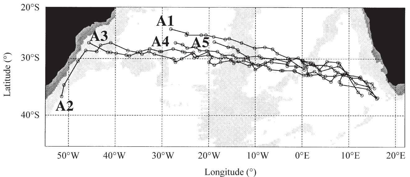
Figure 9. Drift paths of the five selected Agulhas eddies generated during the 5-year experiment. Circles indicate the positions of the eddies at 32-day intervals. Regions where depth of the ocean is less than 3900 m are coloured in grey.
