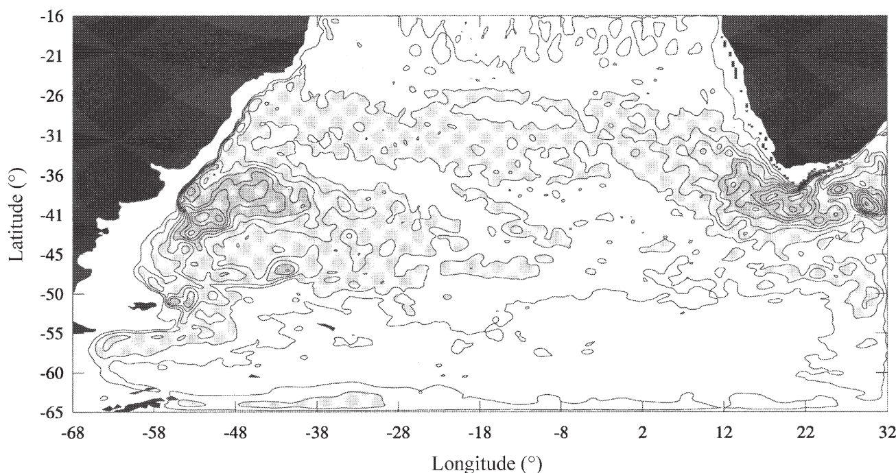
Figure 5. Standard deviation of the annual mean anomalies of the upper-layer circulation. Values larger than 2/5 \text{ Sv} are coloured in light/dark grey respectively. Contour interval is 1 \text{ Sv} .
