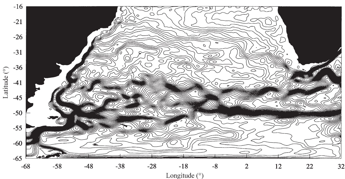
Figure 1. Mean stream function in the upper 300 m of the South Atlantic ocean circulation from the experiment (contour interval is 1 Sv).
