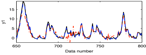
(a) The real output without the measurement noise (solid line) with the outputs of quadratic system (dashed line) and NNOE model (dash-dotted line), and their errors.
