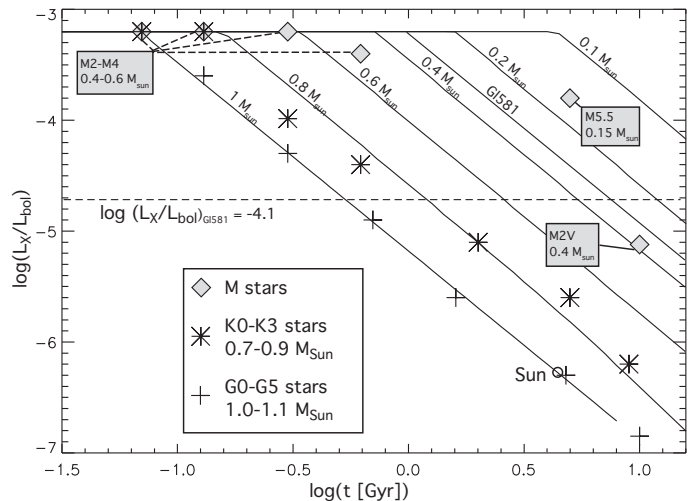
Fig. 5. The plot shows the evolution of the ratio between the X-ray and bolometric luminosities as a function of age for stars of different masses. The solid lines represent semi-empirical laws, while symbols give observed values for G (+), K (*) and M (◇) stars. The dashed line gives the upper limit for the value of \log(L_X/L_{\text{bol}}) in the case of Gl 581, for which there is no ROSAT detection.
