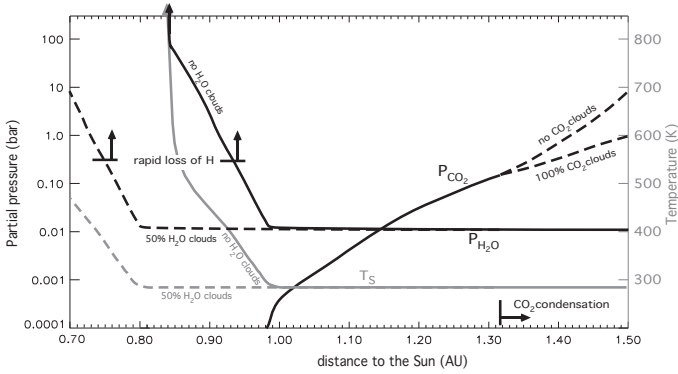
Fig. 1. The \text{CO}_2 and \text{H}_2\text{O} pressure and the mean surface temperature of a habitable planet are shown as a function of the orbital distance. The diagram gives P_{\text{CO}_2} and P_{\text{H}_2\text{O}} (left y-axis) and T_s (grey, right y-axis) of an Earth-like planet across the inner part of the HZ around the present Sun. At orbital distances larger than \sim 0.98 AU, T_s is assumed to be fixed at 288 K (its current value on Earth) by the carbonate-silicate cycle, which is obviously an idealized picture. Beyond 1.3 AU, \text{CO}_2 condenses in the atmosphere and the required level of \text{CO}_2 depends on the coverage by \text{CO}_2 -ice clouds. The pressure of \text{H}_2\text{O} and T_s in the inner HZ is calculated for a cloud-free atmosphere and 50% cloud cover and assuming a reservoir of water that contains (as on Earth) more than the equivalent of 220 bars of \text{H}_2\text{O} .
