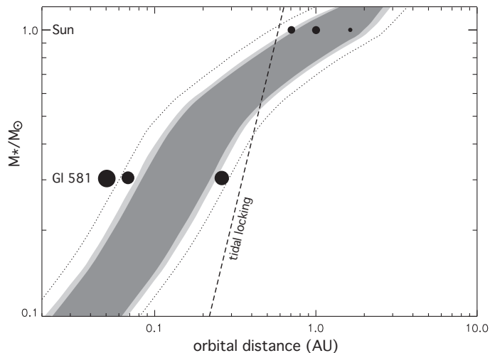
Fig. 3. The orbital region that remains continuously habitable during at least 5 Gyr is shown as a function of the stellar mass. The darker area is defined by the empirical “early Mars” and “recent Venus” criteria. The light grey region gives the theoretical inner (runaway greenhouse) and outer limits with 50% cloudiness, with H 2 O and CO 2 clouds, respectively. The dotted boundaries correspond to the extreme theoretical limits, found with 100% cloud cover. The dashed line indicates the distance at which a 1 M_{\oplus} planet on a circular orbit becomes tidally locked in less than 1 Gyr.
