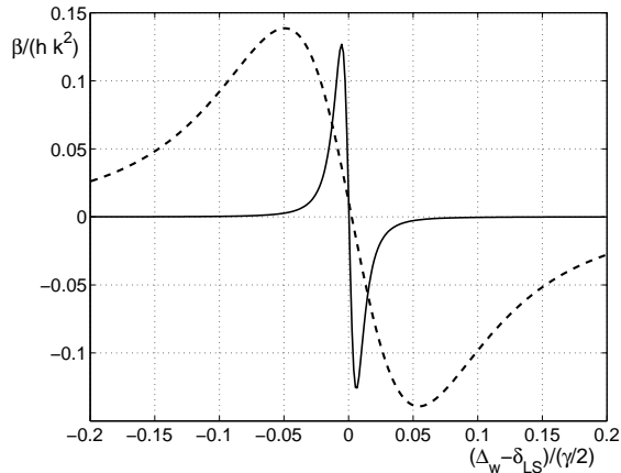
FIG. 5: Damping factor \beta in units of \hbar k^2 , versus the relative detuning of the weak transition from the light-shift. \text{Ca}^+ wavelengths are used ( \lambda_w = 732 nm and \lambda_{st} = 866 nm) and \gamma/2\pi = 20 MHz. The two curves are for different values of \Omega_w/2\pi : 0.1 MHz (solid line), 1 MHz (dashed line), \Delta_{st}/2\pi is fixed to -10\gamma and \Omega_{st} is chosen to obtain the maximum signal, according to Eq.12.
