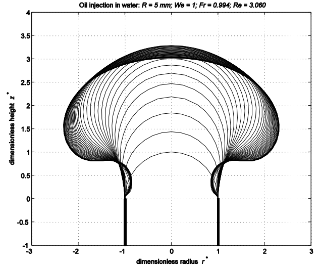
Figure 6. Oil injection in water (superposed frames) for R = 5 mm
