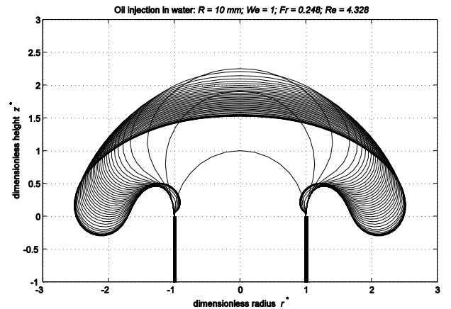
Figure 8. Oil injection in water (superposed frames) for R = 10 mm
