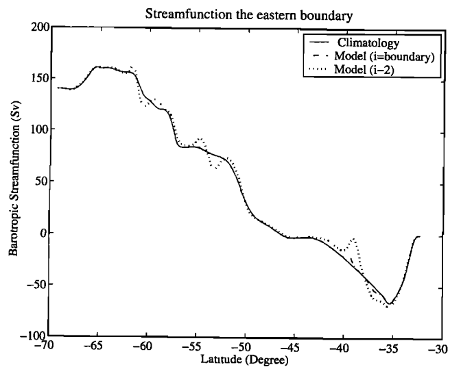
Figure 8. Profiles of barotropic stream function at the eastern boundary (Sv). The solid line is the climatology derived from the WOCE I6 section (see section 2). The dashed line is an instantaneous profile at the boundary, the dotted line an instantaneous profile two grid points away from the boundary.
