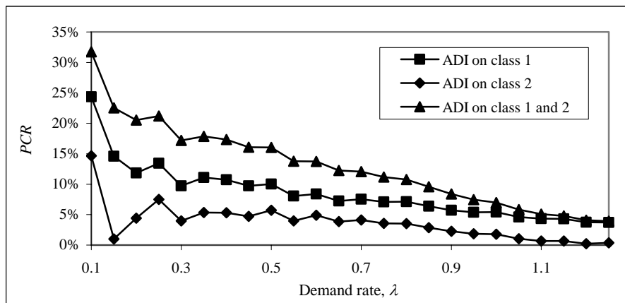
(c) The effect of demand rate ( \lambda_1 = \lambda_2 = \lambda , c_1 = 200 , c_2 = 50 , p_1 = p_2 = 1 , \nu_1 = \nu_2 = 0.1 )
