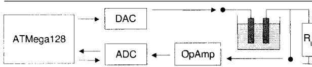
Figure 4. Block diagram
